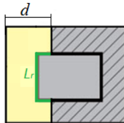
Figure 6: Resonance length.
