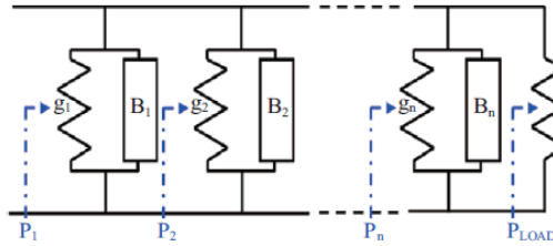
Figure 3: Circuital model of a slotted waveguide on the narrow face.
