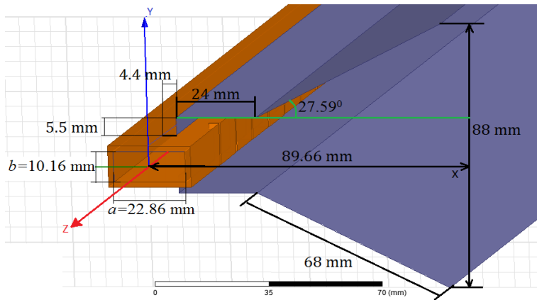
Figure 9: Reflector dimensions.
